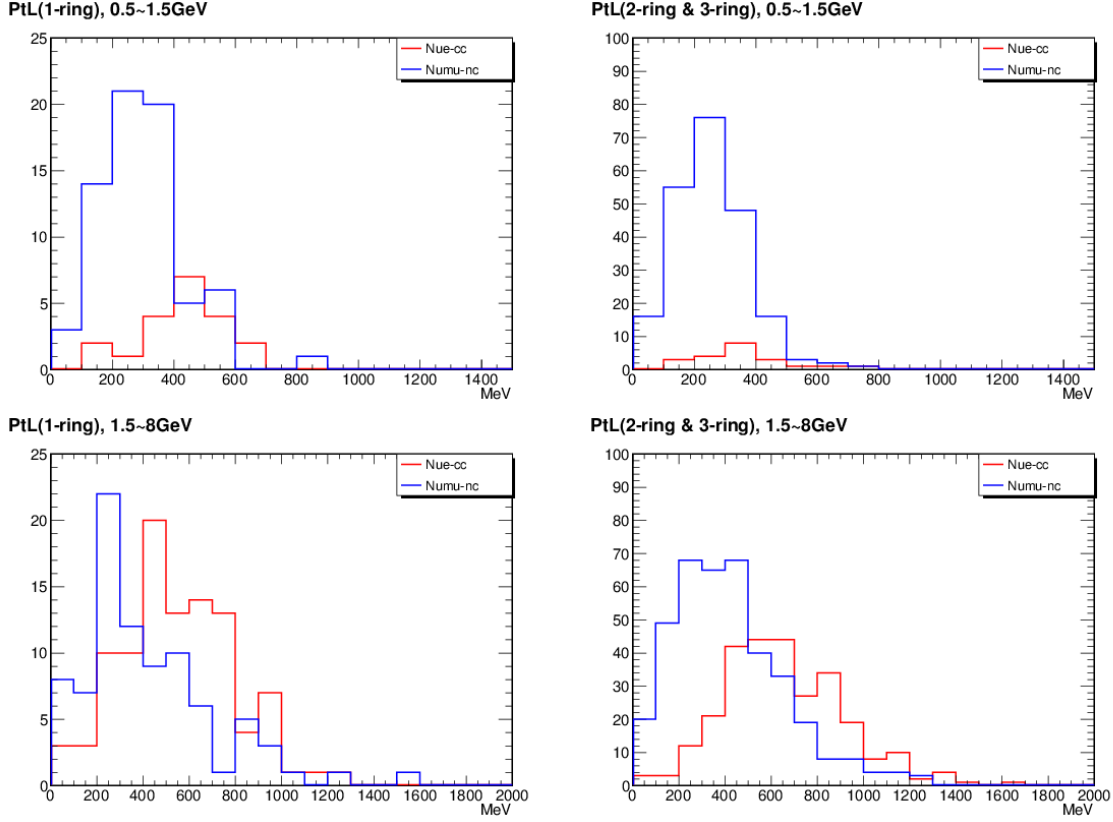
Figure 2.10 P_t^L distribution of 1R, 2R and 3R events in 0.5 ~ 1.5 GeV region and 1.5 ~ 8 GeV region.
