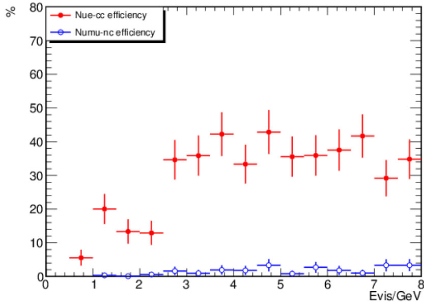
Figure 2.14 2-ring and 3-ring event efficiencies of \nu_e -CC and NC
