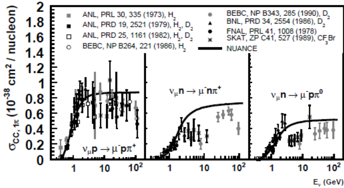
Figure 3.2 Historical measurement of resonance single pion production. The black line represents theoretical calculation using NUANCE using MA = 1.1 \text{ GeV} [23]. (Plot taken from [22])
