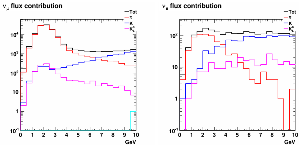
Figure 4.7 \nu_\mu (left) and \nu_e (right) flux composition in \text{NO}\nu\text{A} near detector.
