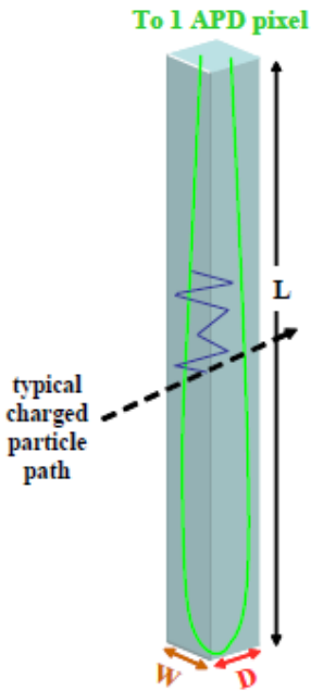
Figure 4.2 The \text{NO}\nu\text{A} PVC cell containing liquid scintillator and a wavelength-shifting fibers(WSF).
