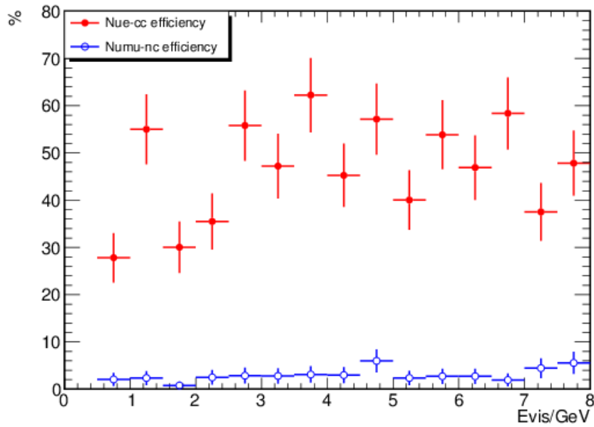
Figure 2.15 Cumulative efficiencies of \nu_e -CC and NC.
